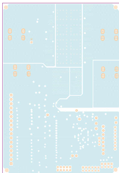
Figure 51: Mid-Layer 1
