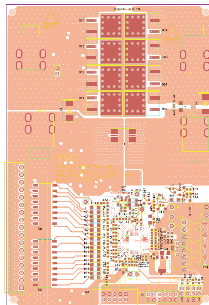
Figure 50: Top Layer
