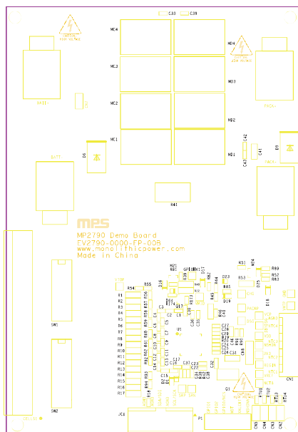
Figure 49: Top Silk
