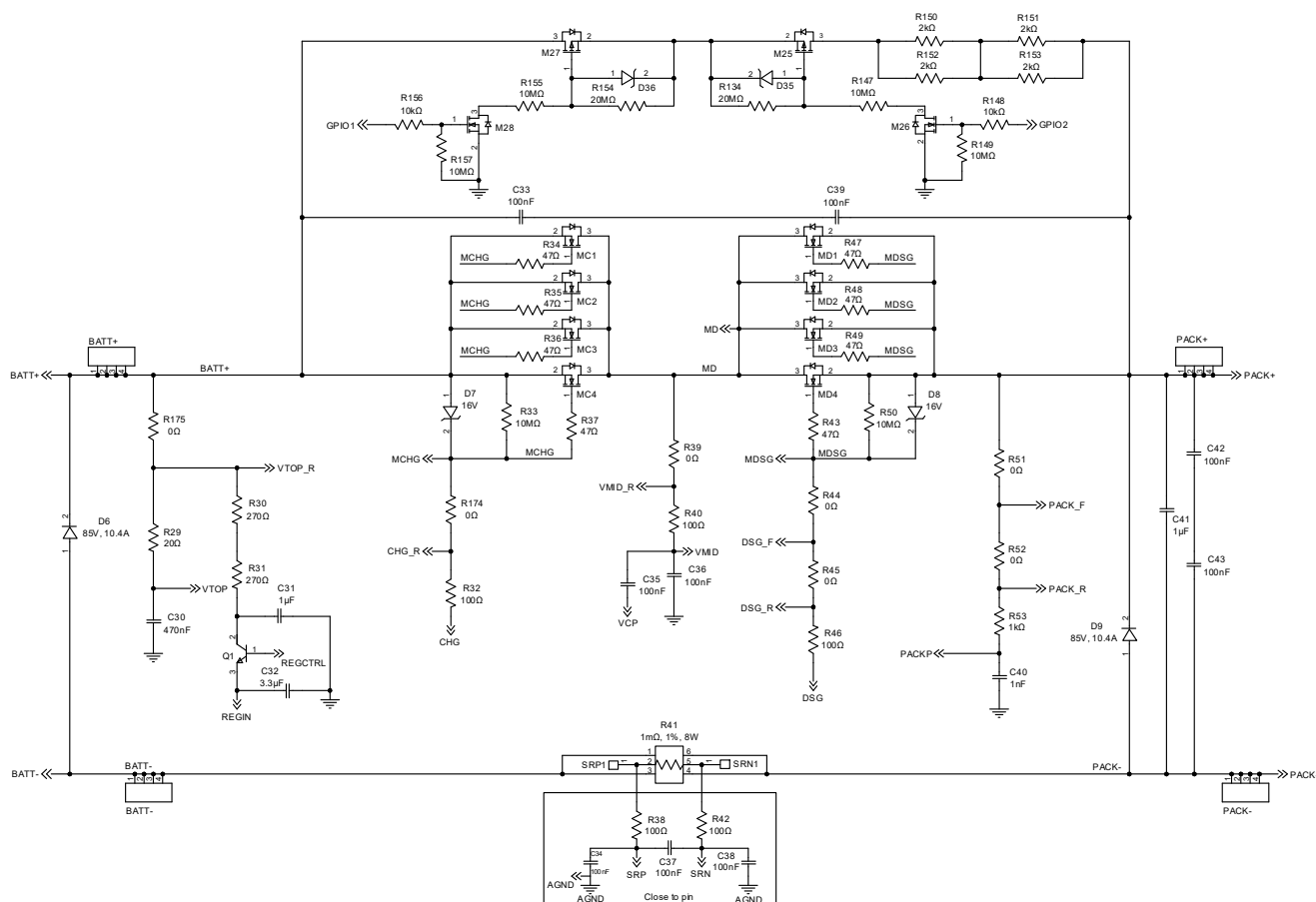
Figure 46: Evaluation Board Schematic (Power Path)
