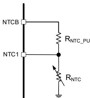
Figure 42: NTC Functional Block Diagram
