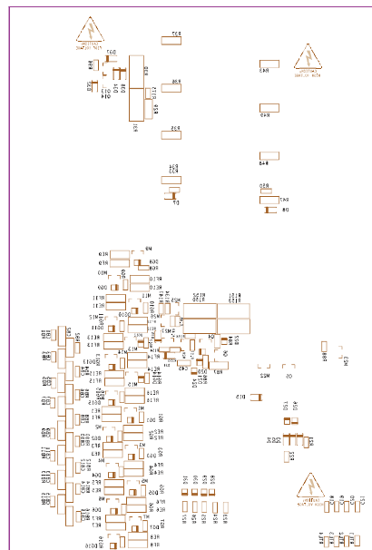
Figure 54: Bottom Silk
