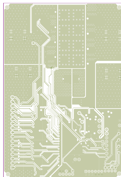
Figure 52: Mid-Layer 2
