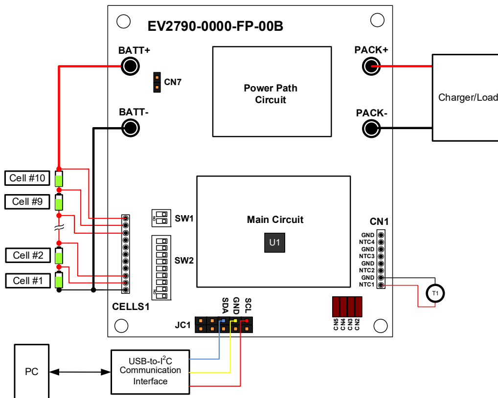
Figure 4: Equipment Set-Up for the MP2790DFP-0000 with a Battery Pack
